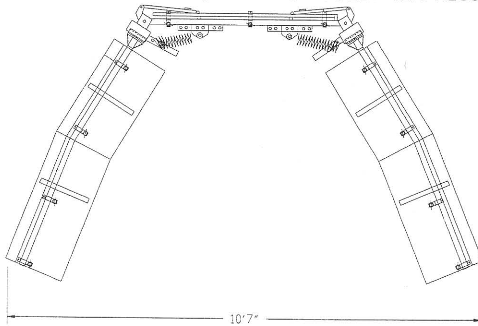
RANDELL WEED WING, TOP VIEW FULLY COMPRESSED
